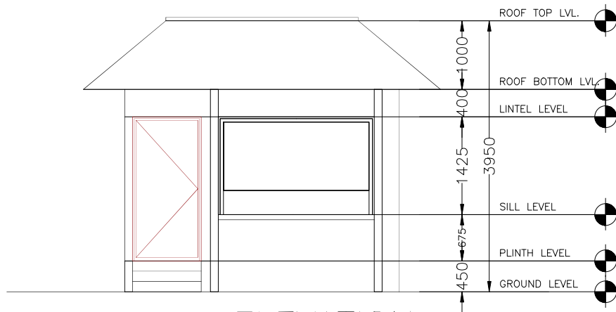
FRONT ELEVATION
