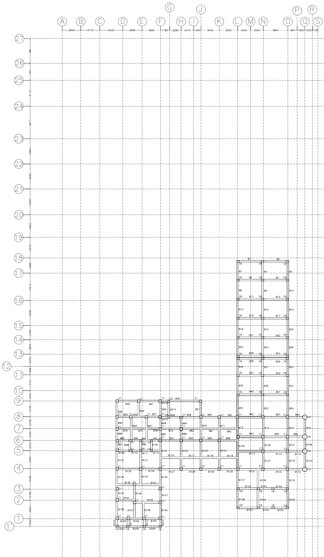
BEAM & SLAB LAYOUT AT LEVEL -10.2M
