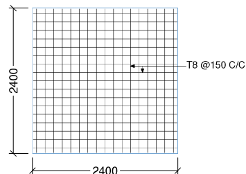
PLAN OF FOOTING/ BED
