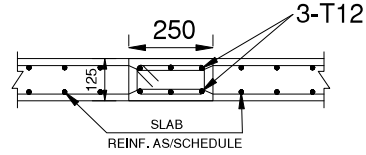
CONCEALED BEAM DETAILS (250X125)
