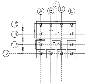
FOUNDATION LAYOUT PLAN B.O.F AT LEVEL -5.0M FROM E.G.L
