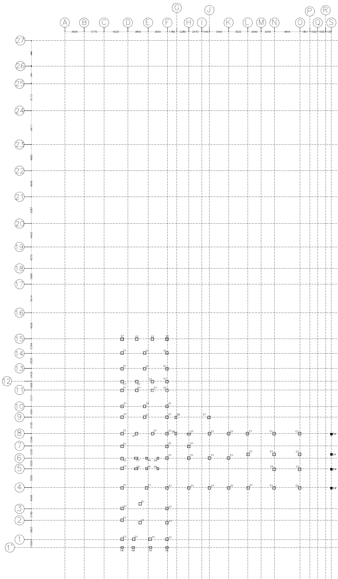
COLUMN LAYOUT AT LEVEL -3.0M
