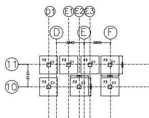
FOUNDATION LAYOUT AT -8.6 M DEPTH
