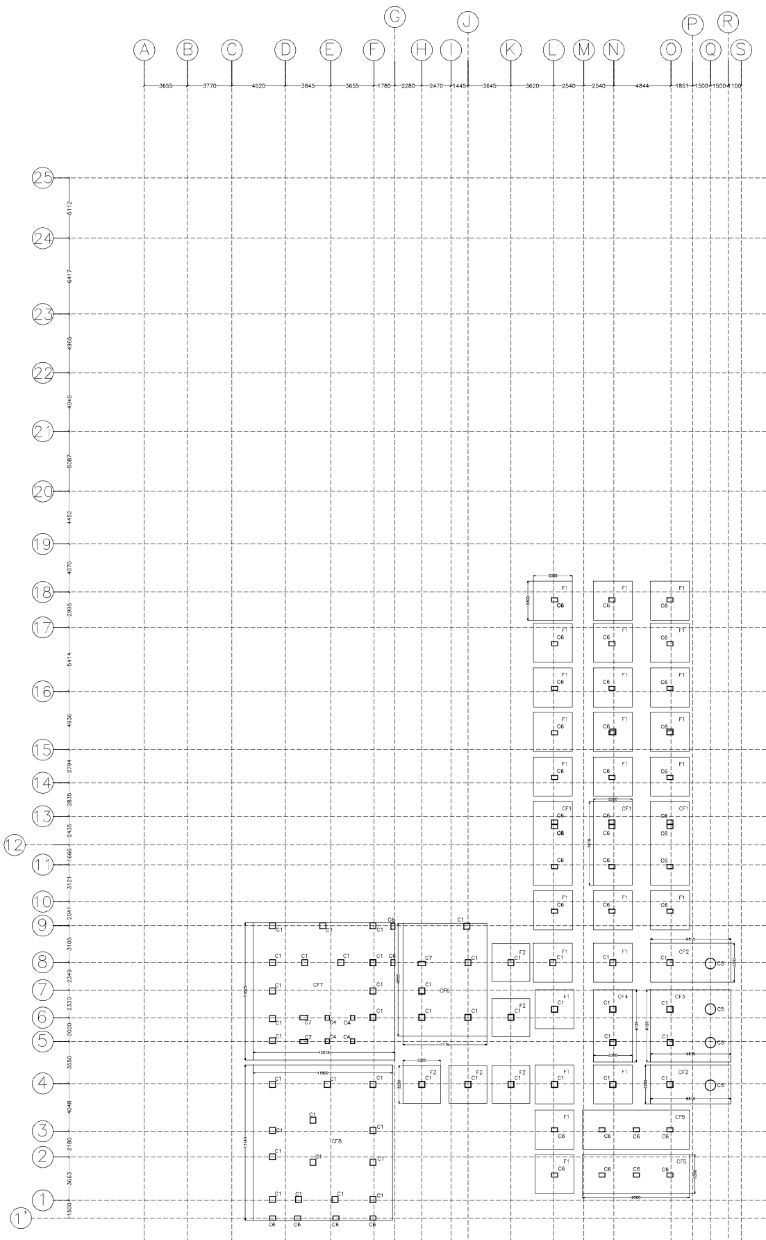
FOUNDATION LAYOUT PLAN B.O.F AT LEVEL -12.2M FROM E.G.L
