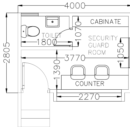
SECURITY KIOSK FLOOR PLAN
