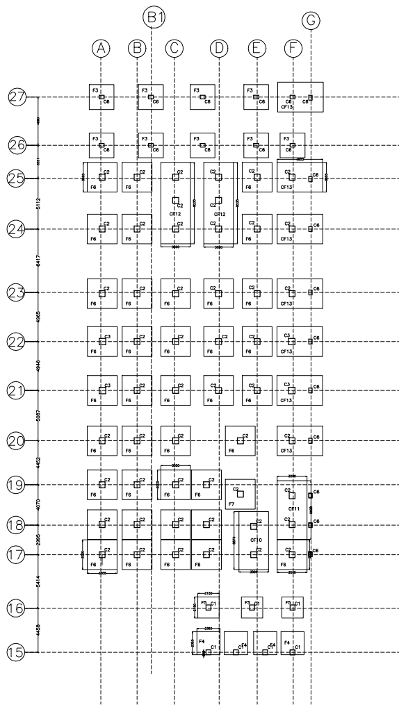
FOUNDATION LAYOUT PLAN B.O.F AT LEVEL -2.0 M FROM E.G.L
