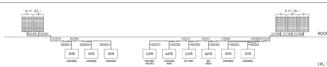
REFRIGERANT PIPING SCHEMATIC DIAGRAM
