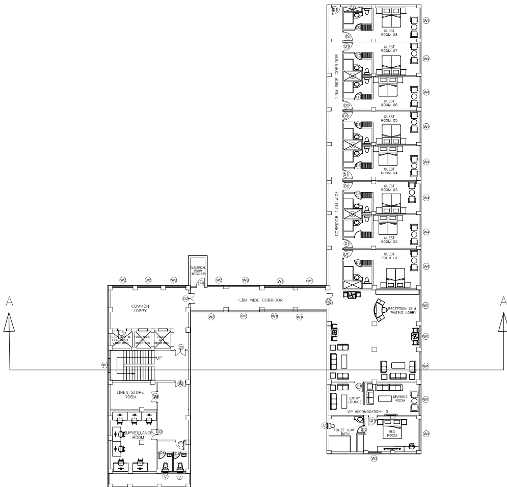
LVL.4 FLOOR PLAN TOTAL AREA-752.2 SQ.M.
