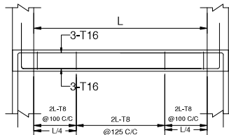
BEAM DETAILS (250X300)
